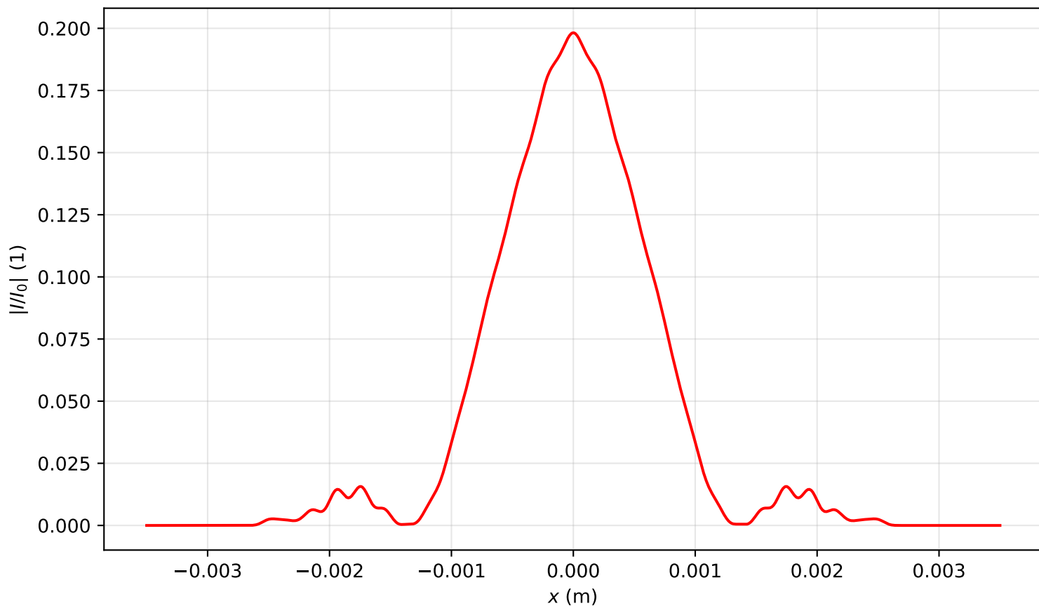
Intensity profile I(x, y = 0, z = 1.433)/I_0 , Pin=2.0Pcr, artificial time
